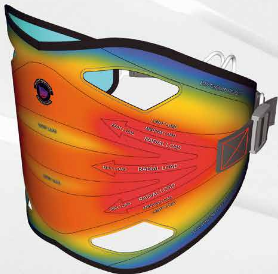
MARK I LOAD PLATE
